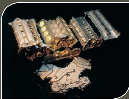
A complete set of castings for an Indy Racing League Engine
